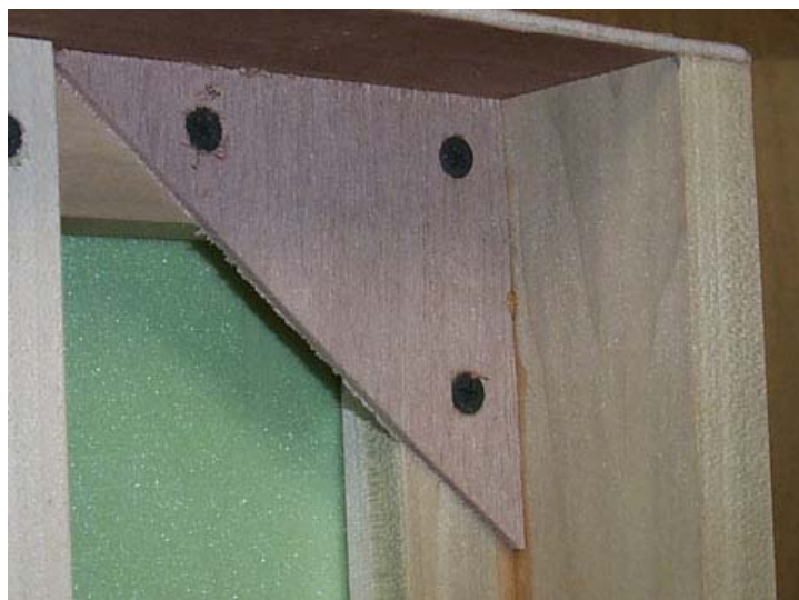
Now, after ensuring that the module is square, corner gussets are glued and screwed to the stiffeners to eliminate racking.
